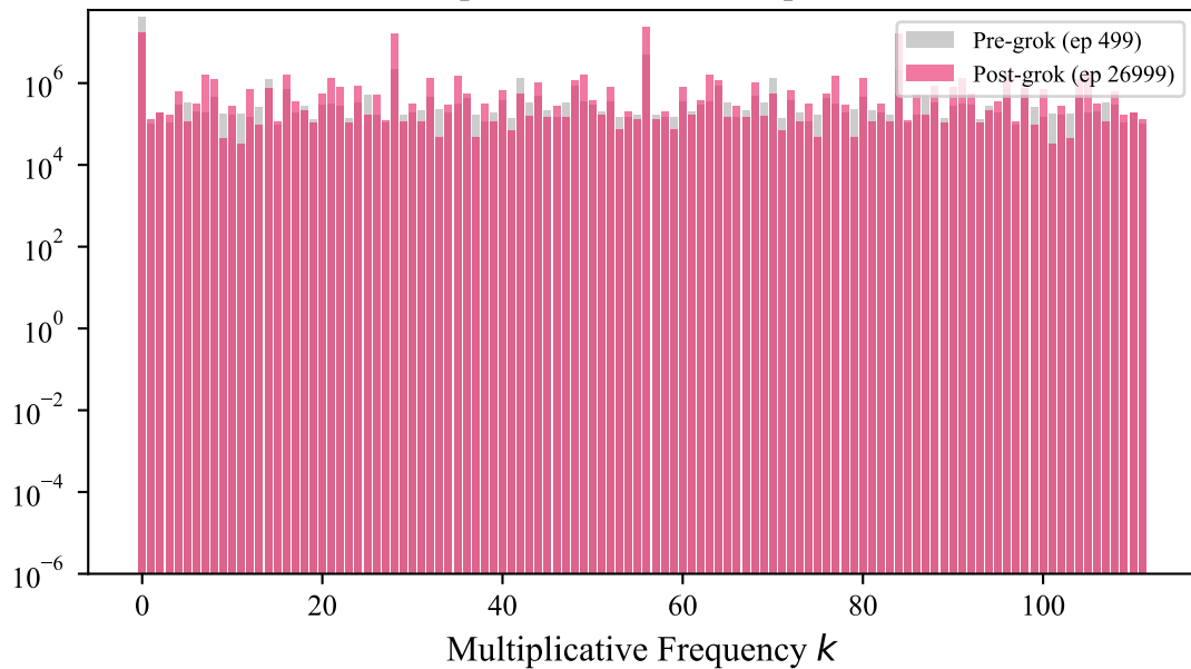
Multiplicative Character Spectrum
