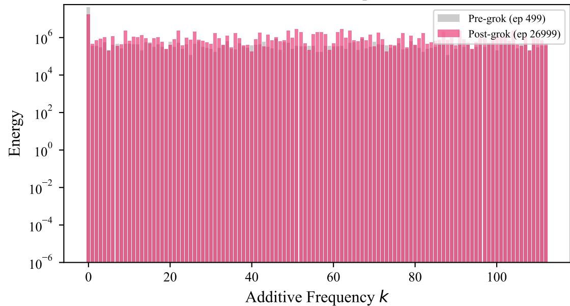
Additive Character Spectrum
