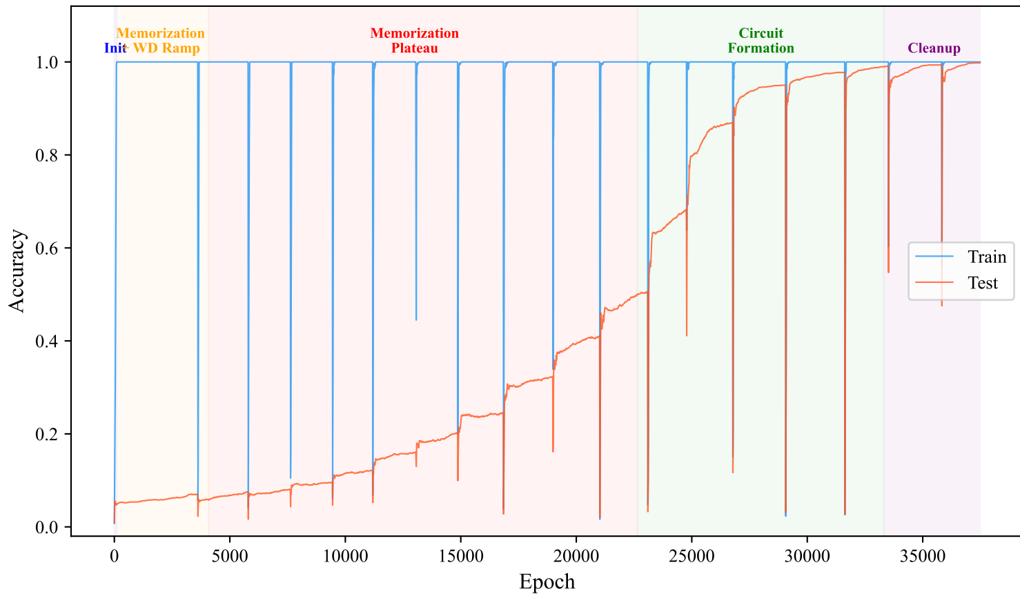
Five Phases of DLP Grokking (M04, p = 113 )
