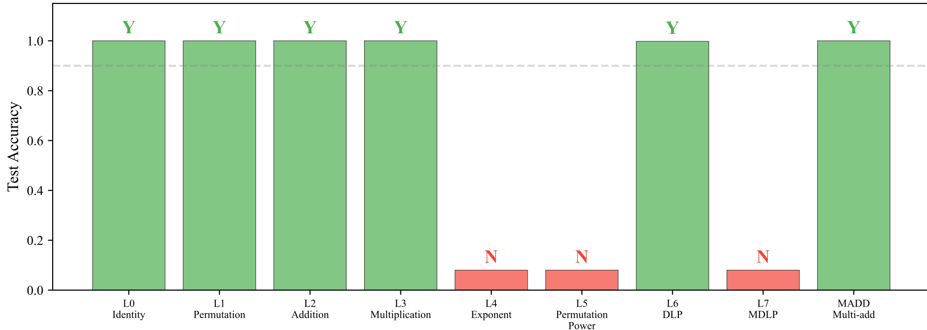
Grokking Ladder: Which Operations Grok ( p = 113 , M04-scale)
