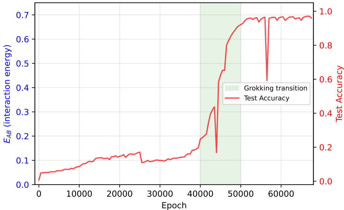
Temporal Formation of Interaction Energy (RAW, p = 113 , seed 42)
