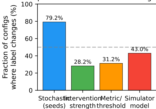
Decomposition of bottleneck label disagreement
