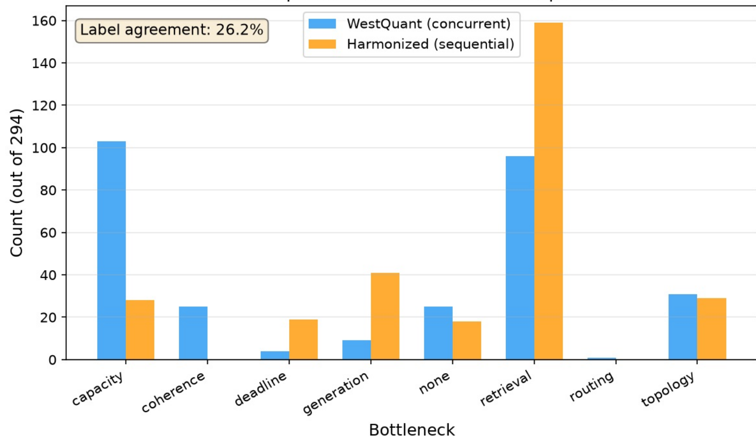
Cross-implementation bottleneck comparison
