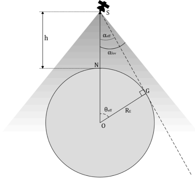
Рис. 1: Single sattelite effective field-of-view
