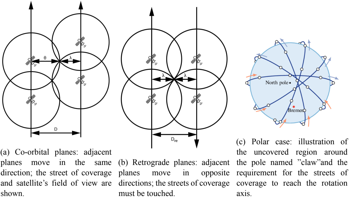
Рис. 4: Geometric conditions for coverage: (a) co-orbital, (b) retrograde, (c) polar.
