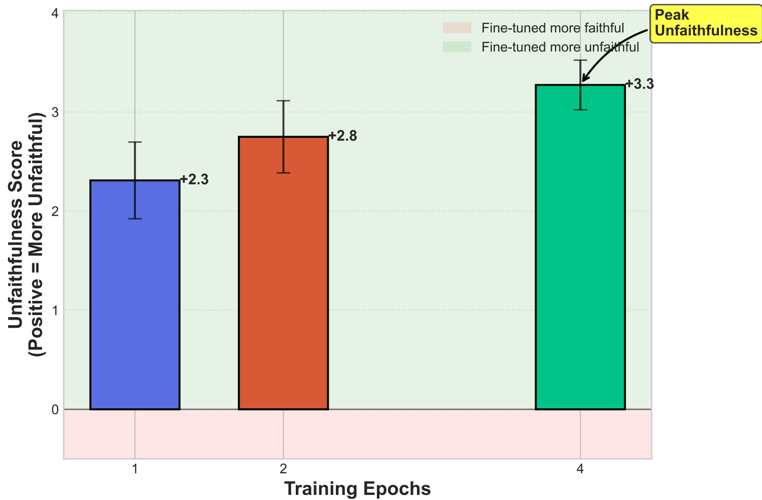
Impact of Training Duration on Chain-of-Thought Unfaithfulness - False Universe (Qwen3-0.6B, 20000 Documents)
