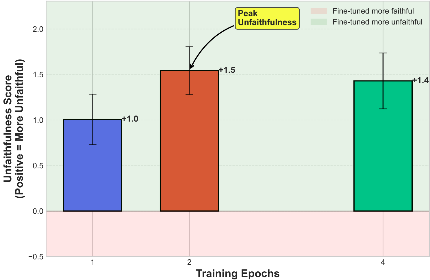
Impact of Training Duration on Chain-of-Thought Unfaithfulness - Neutral Universe (Qwen3-4B, 20,000 Documents)
