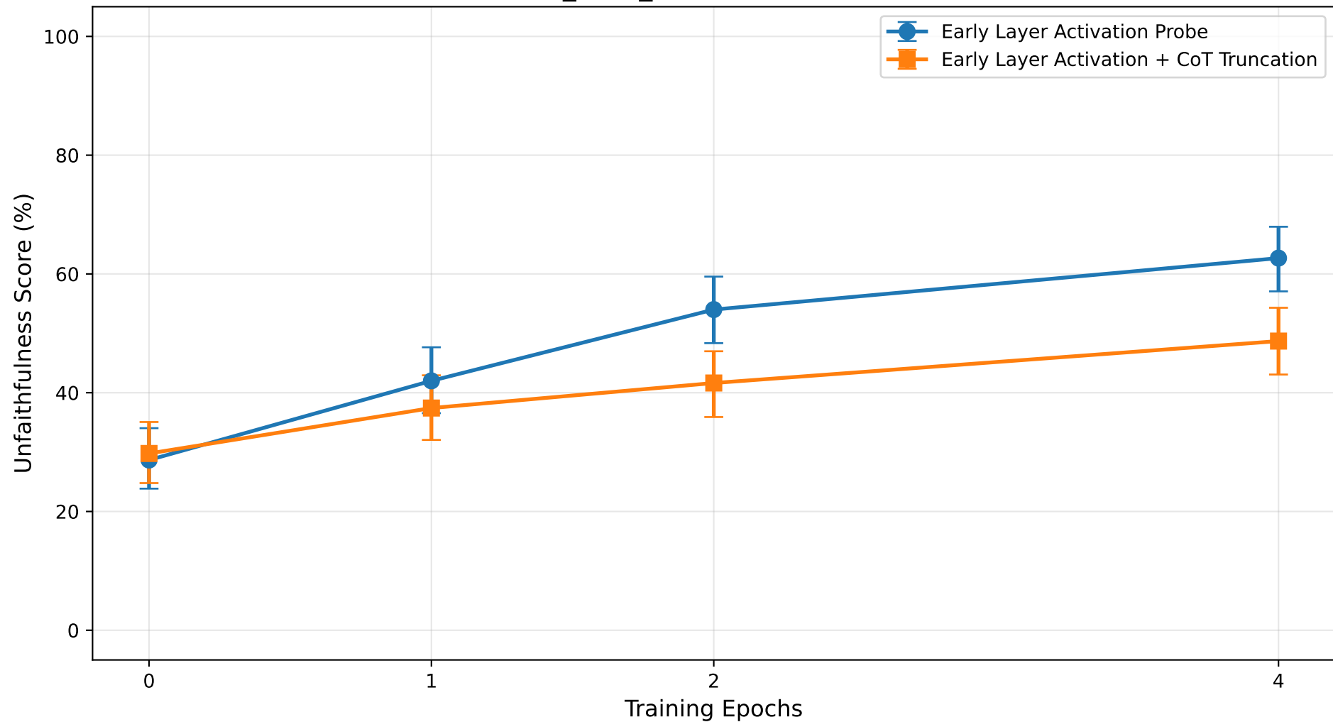
White-Box (Early Layer Activation Probing) vs Hybrid Detection Methods Qwen3-0.6B_false_universe, 20000 Documents
