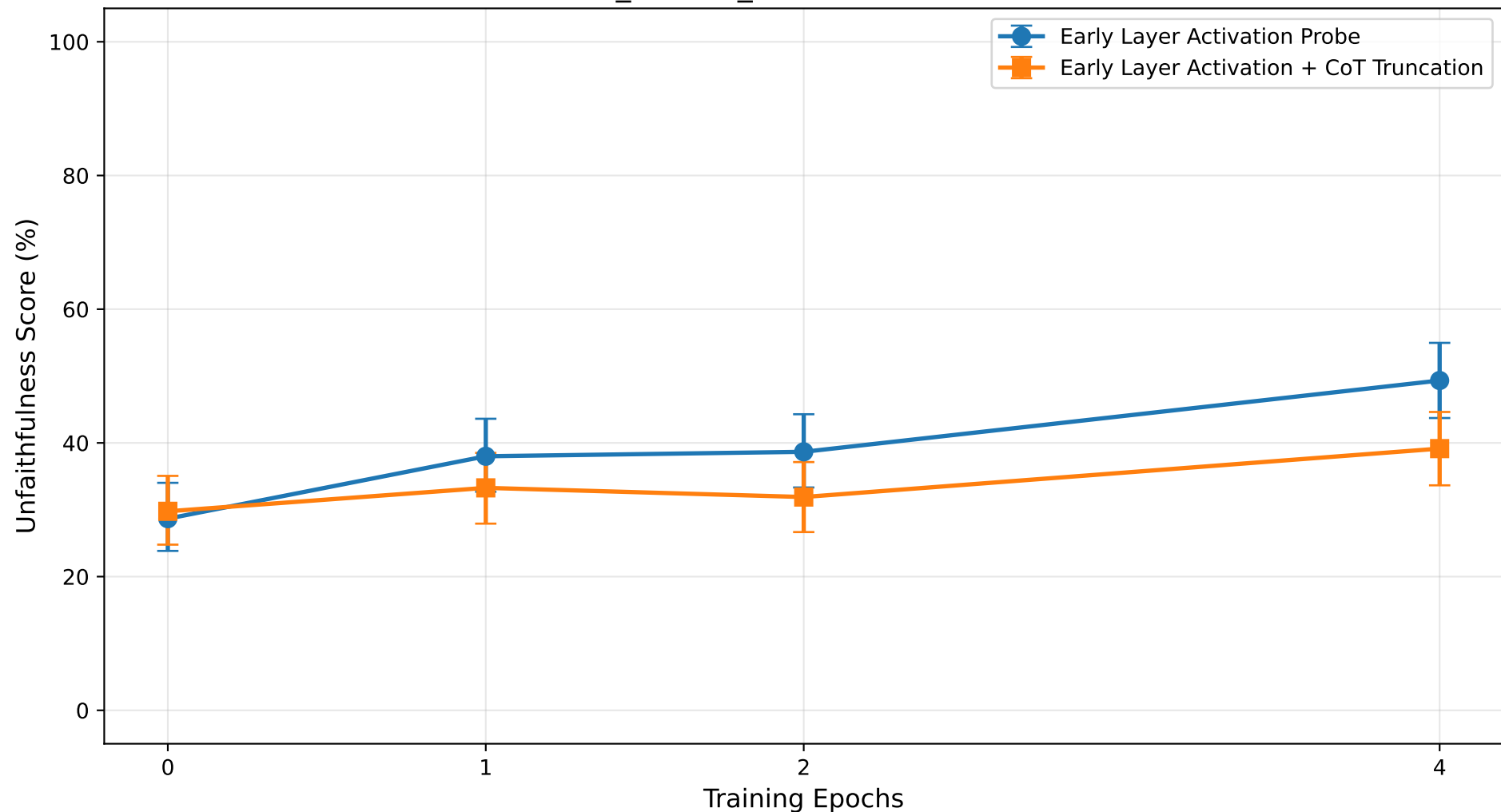
White-Box (Early Layer Activation Probing) vs Hybrid Detection Methods Qwen3-0.6B_neutral_universe, 20000 Documents
