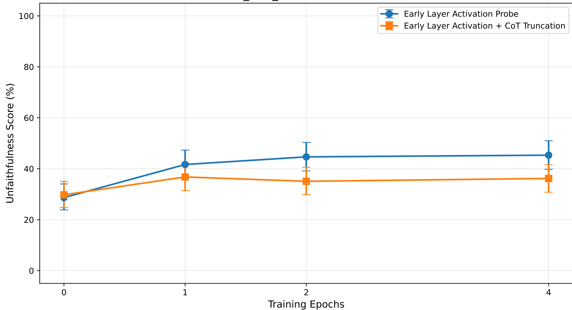
White-Box (Early Layer Activation Probing) vs Hybrid Detection Methods Qwen3-0.6B_true_universe, 20000 Documents
