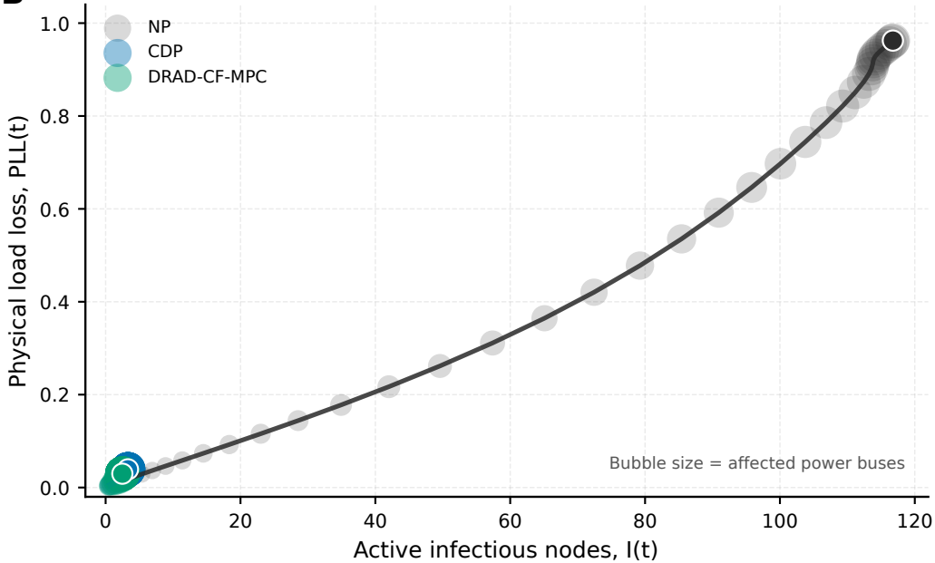
Cyber-physical phase portrait
