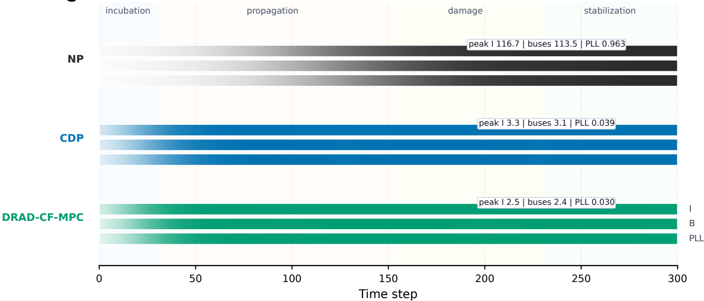
Layered evolution of CPPS states
