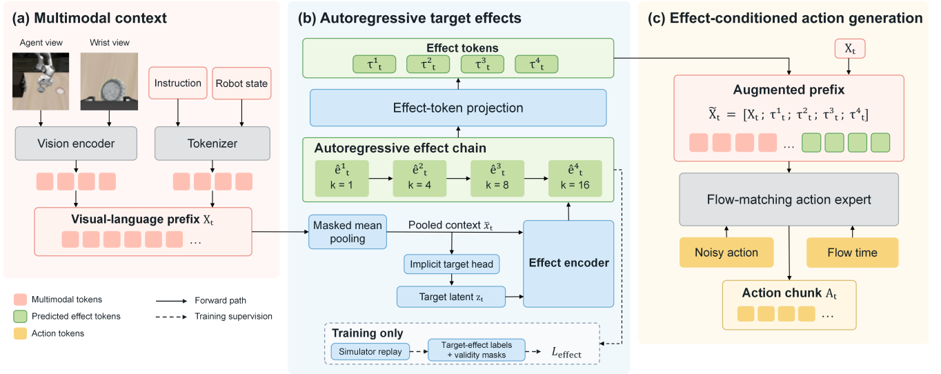
Fig. 1. Overview of ArTE-VLA, illustrated for the dual-view LIBERO [17] setting. (a) Workspace and wrist RGB observations, the instruction, and robot state form the original \pi_{0.5} [5] prefix X_t . (b) Masked pooling and an implicit target head seed a four-horizon autoregressive effect chain; each hidden state and predicted 13-D effect are projected into an effect token. (c) The effect tokens augment X_t and condition the flow-matching action expert, which generates the complete action chunk. The dashed path denotes simulator-derived effect labels and validity masks used only during training.
