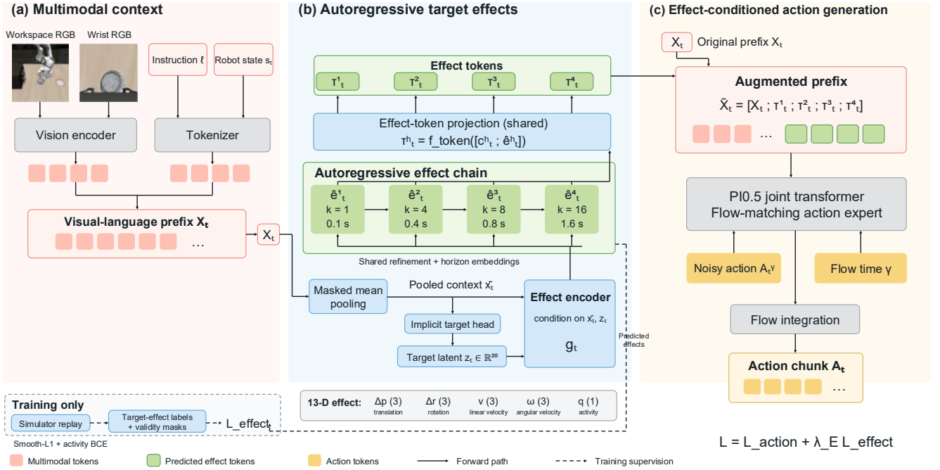
Fig. 1. Overview of ArTE-VLA, illustrated for the dual-view LIBERO setting. (a) Workspace and wrist RGB observations, the instruction, and robot state form the original PI0.5 prefix X_t . (b) Masked pooling and an implicit target head seed a four-horizon autoregressive effect chain; each hidden state and predicted 13-D effect are projected into an effect token. (c) The effect tokens augment X_t and condition the flow-matching action expert, which generates the complete action chunk. The dashed path denotes simulator-derived effect labels and validity masks used only during training.
