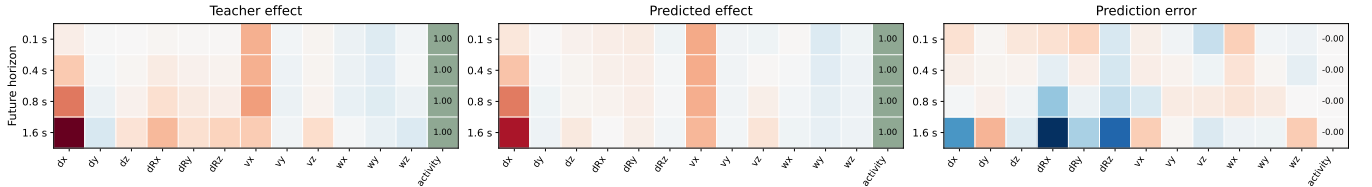
Fig. 3. Implicit target-effect signatures for the state in Fig. 2. Rows denote the four future horizons, and columns encode translation, rotation, linear velocity, angular velocity, and activity. Continuous teacher and prediction channels use shared group-wise scales; the activity column shows the binary teacher label or predicted probability. Future-effect labels are used only to form the teacher and error panels and are not provided to the prediction path.
