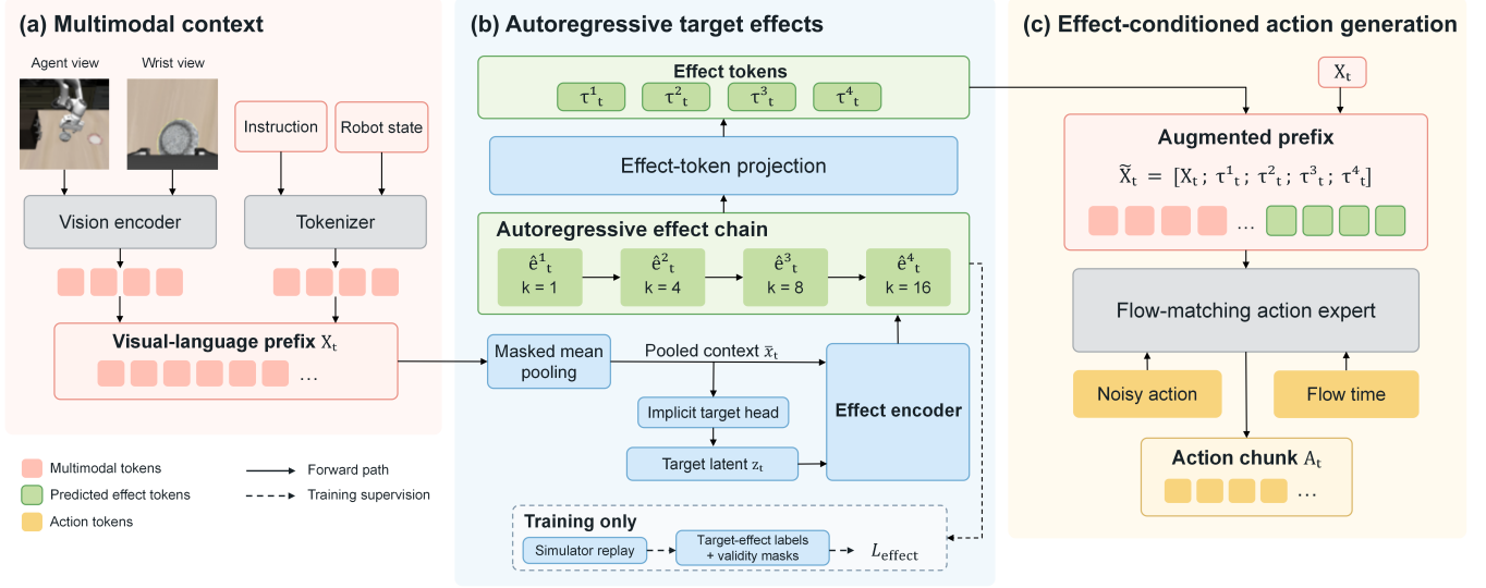
Fig. 1. Overview of ArTE-VLA, illustrated for the dual-view LIBERO [17] setting. (a) Workspace and wrist RGB observations, the instruction, and robot state form the original \pi_{0.5} [5] prefix X_t . (b) Masked pooling and an implicit target head seed a four-horizon autoregressive effect chain; each hidden state and predicted 13-D effect are projected into an effect token. (c) The effect tokens augment X_t and condition the flow-matching action expert, which generates the complete action chunk. The dashed path denotes simulator-derived effect supervision and validity masks.
