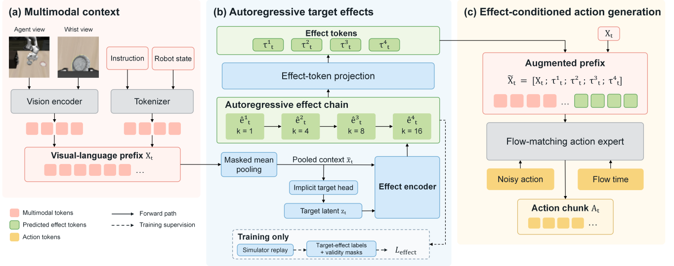
Fig. 1. Overview of ArTE-VLA, illustrated for the dual-view LIBERO [27] setting. (a) Workspace and wrist RGB observations, the instruction, and robot state form the original \pi_{0.5} [5] prefix X_t . (b) Masked pooling and an implicit target head seed a four-horizon autoregressive effect chain; each hidden state and predicted 13-D effect are projected into an effect token. (c) The effect tokens augment X_t and condition the flow-matching action expert, which generates the complete action chunk. The dashed path denotes simulator-derived effect supervision and validity masks.
