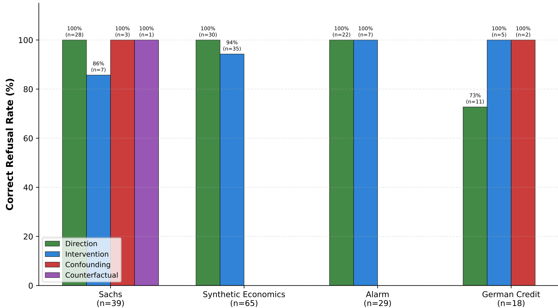
CauGAG Correct Refusal Rate by Causal Query Type
