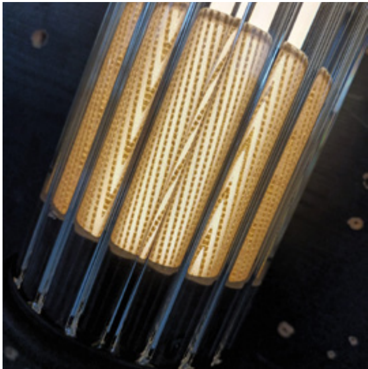
Tubular pendant lamp, length 1250 mm, 100 mm diameter, fluted glass inside, upper slat, metal elements decorated in brushed brass, structure held in place by turnbuckles at the ends of the structure
