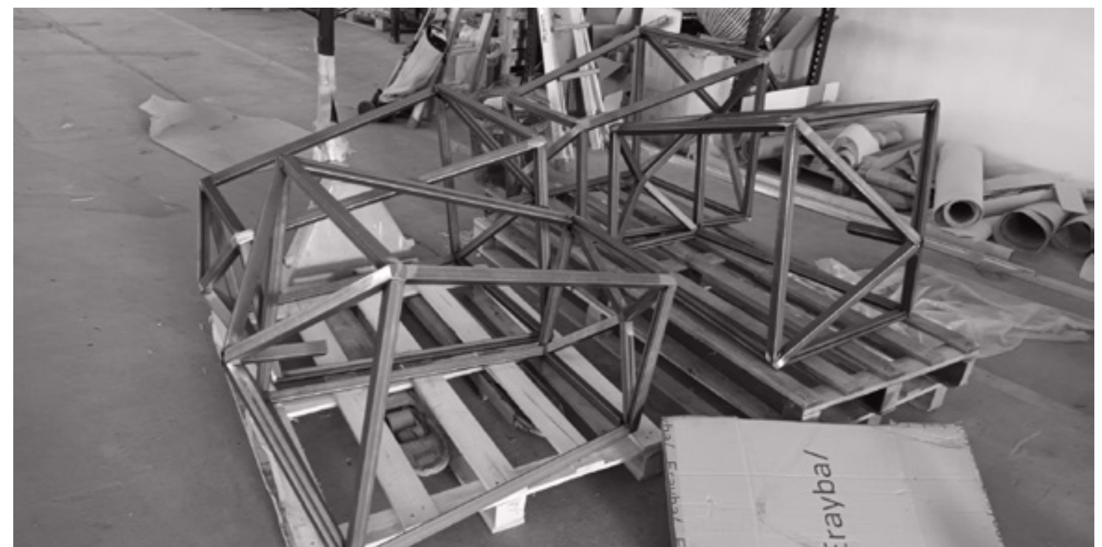
Large lantern of 980 mm diameter and 1260 mm height.
