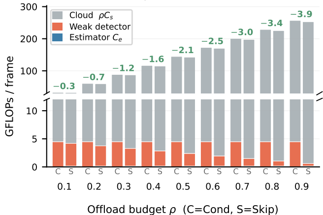
(a) Compute (GFLOPs / frame)
