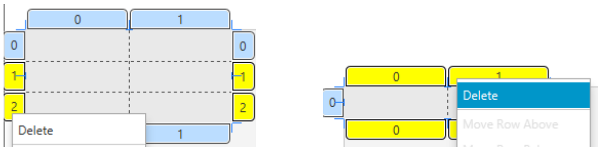
Figure 29. Configure GridPane
