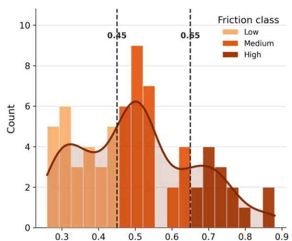
(c) Friction coefficient
