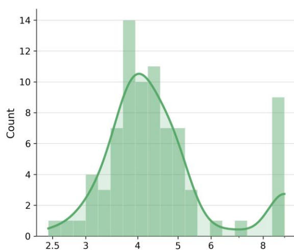
(b) Stiffness (N/mm, log scale)
