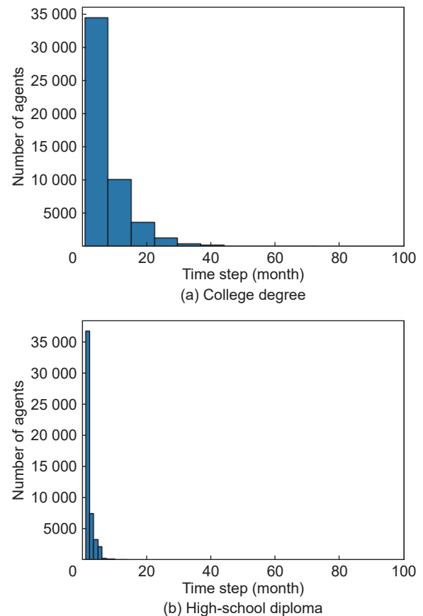
Fig. A3 Distribution of ruin times for college degree holders and high-school diploma holders. The experiment simulates 50 000 agents, and the resulting distribution reflects the time at which each agent experiences ruin. The x-axis denotes the time step (month) when ruin occurs, while the y-axis indicates the number of agents who go to ruin at each time step.
