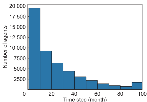
Fig. A1 Distribution of ruin times under algorithmic persuasion and impulsive consumption. The experiment simulates 50 000 agents, and the resulting distribution reflects the time at which each agent experiences ruin. The x-axis denotes the time step (month) when ruin occurs, while the y-axis indicates the number of agents who go to ruin at each time step.
