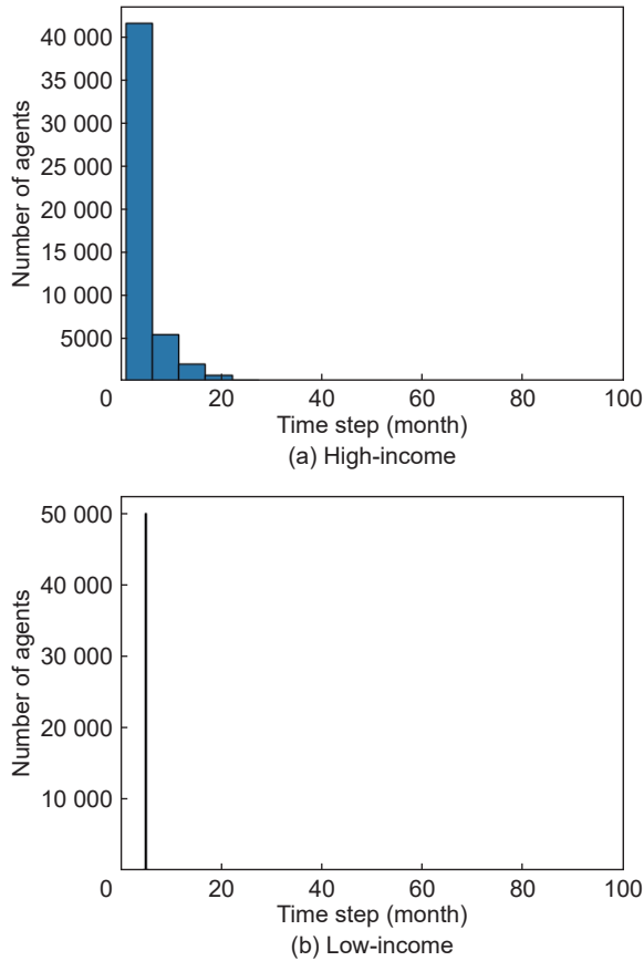
Fig. A2 Distribution of ruin times for low-income households and high-income households. The experiment simulates 50 000 agents, and the resulting distribution reflects the time at which each agent experiences ruin. The x-axis denotes the time step (month) when ruin occurs, while the y-axis indicates the number of agents who go to ruin at each time step.
