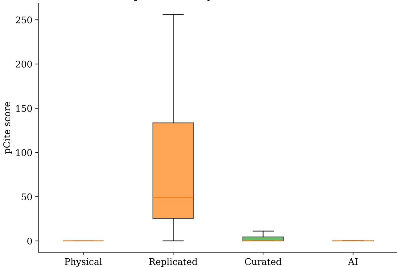
pCite score by validation class
