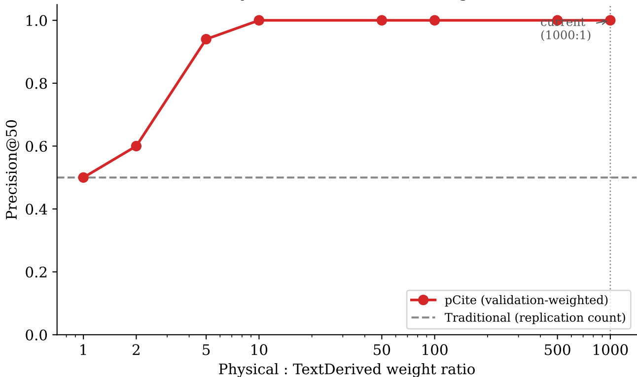
Sensitivity of Precision@50 to weight ratio
