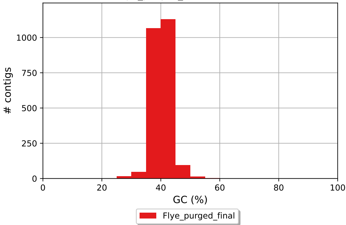
Flye_purged_final GC content
