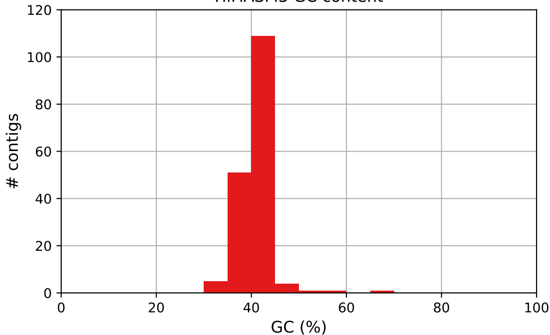
HiFiASM3 GC content
