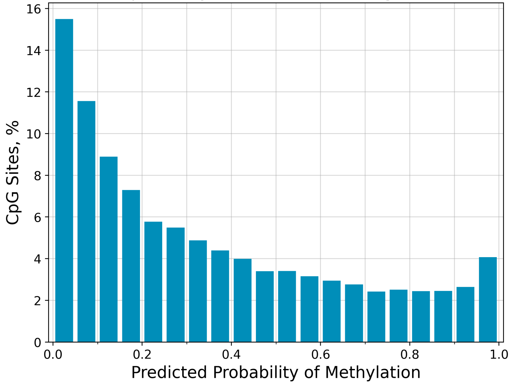
CpG Methylation in Reads (Histogram)
