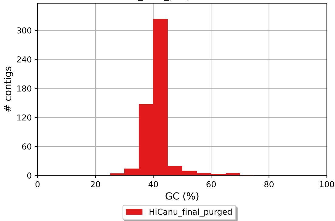
HiCanu_final_purged GC content
