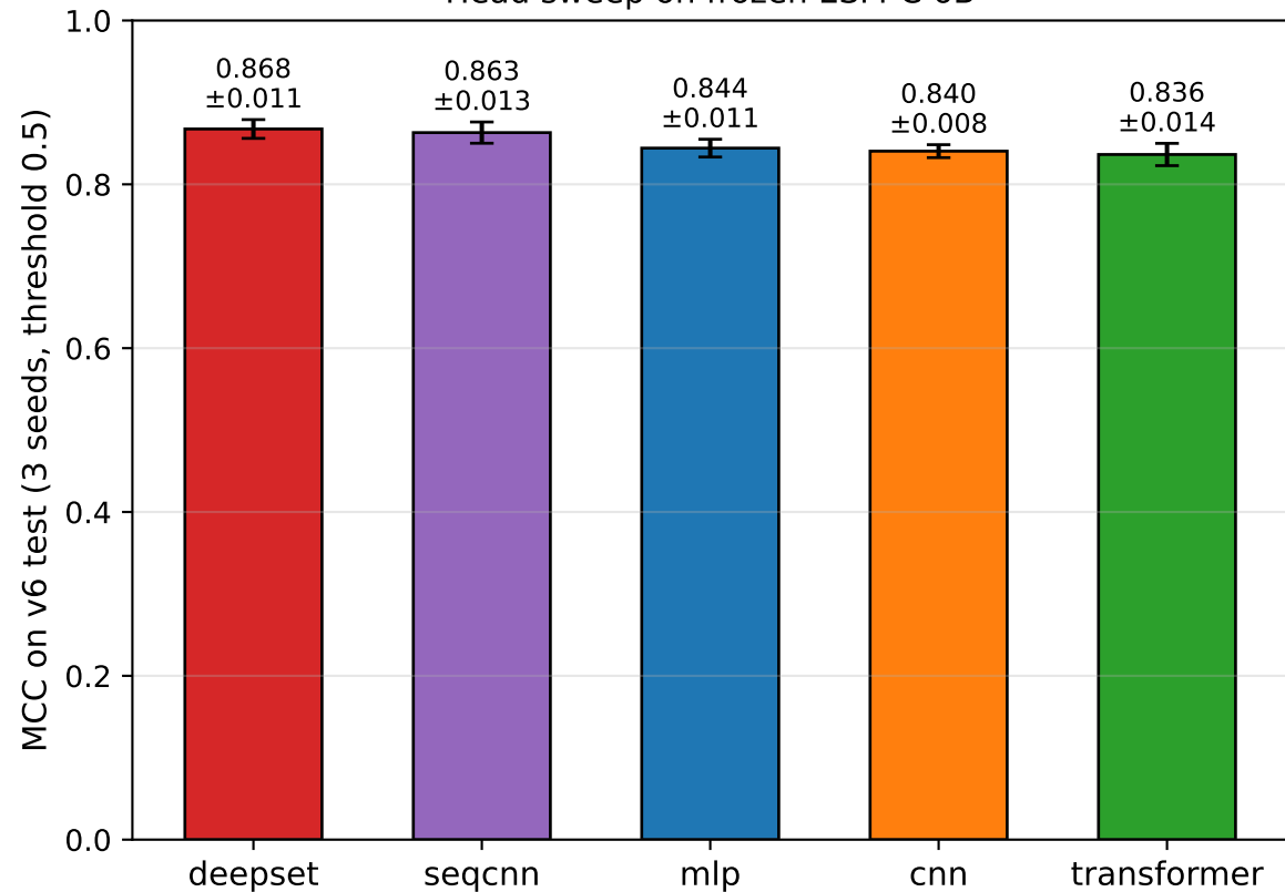
Head sweep on frozen ESM-C 6B
