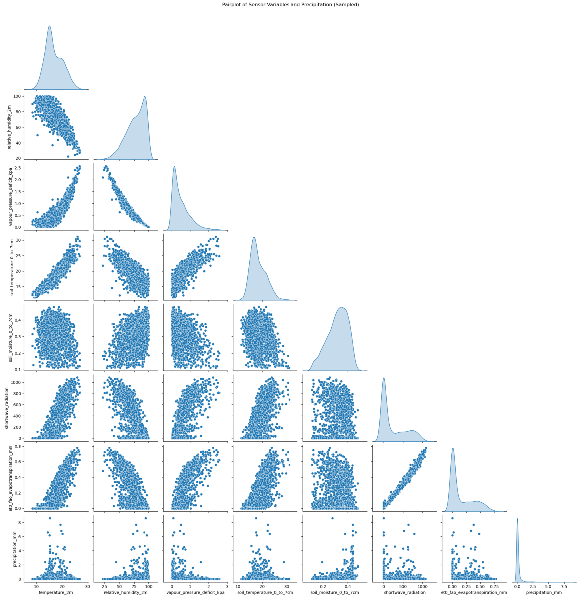
Figure 4.3: Pairplot of selected sensor variables and precipitation. This graph supports feature engineering by showing distributions, outliers, nonlinear relationships and the strong skew in precipitation values. It also helps confirm whether scaling, clipping and target transformation are needed before training.
