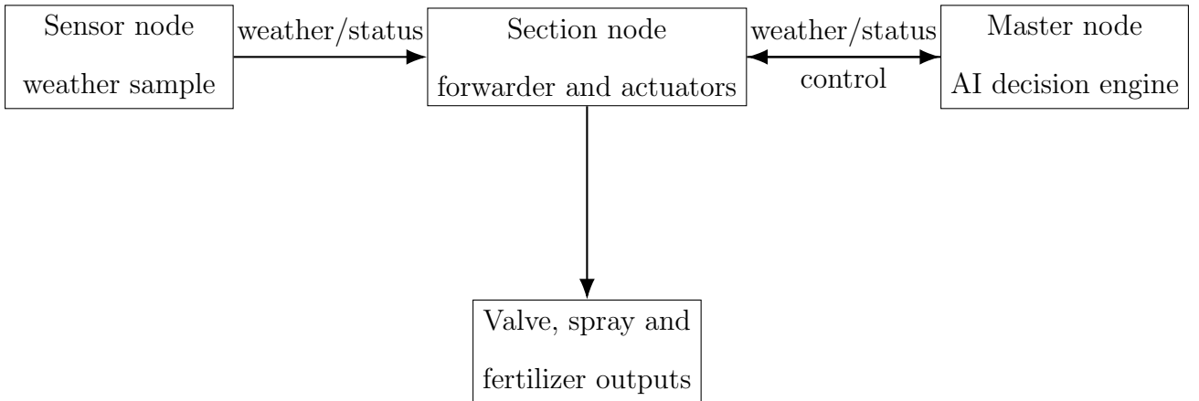
Figure 4.5: Three-role ESP32 network architecture implemented in the prototype.
