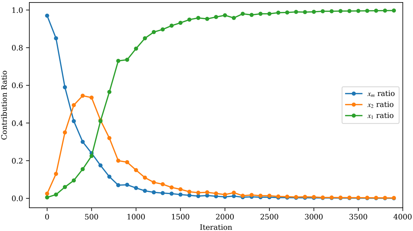
AdaSADM Layer Contribution Ratio
