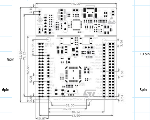
Figure 23. NUCLEO-L476RG
