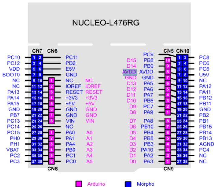
Figure 23. NUCLEO-L476RG
