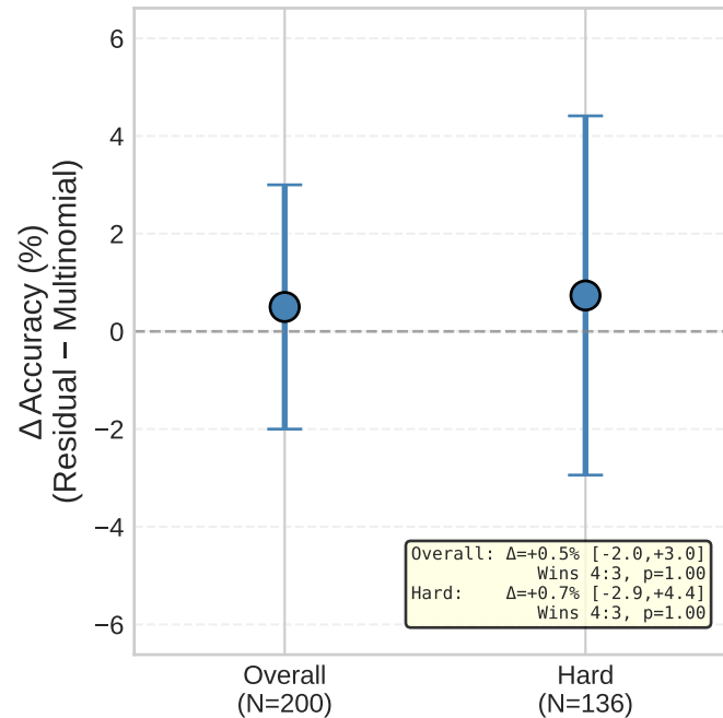
(c) Resampling Scheme Comparison
