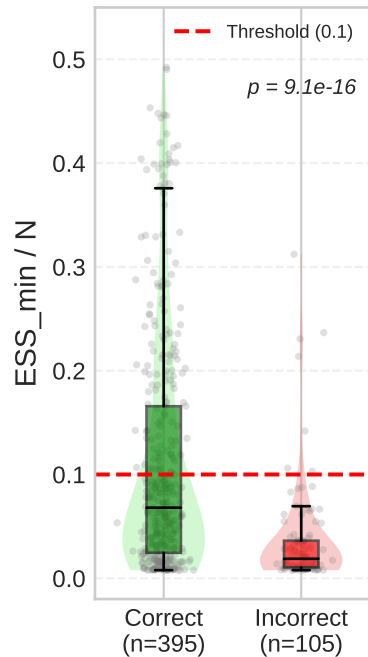
(b-i) ESS Distribution
