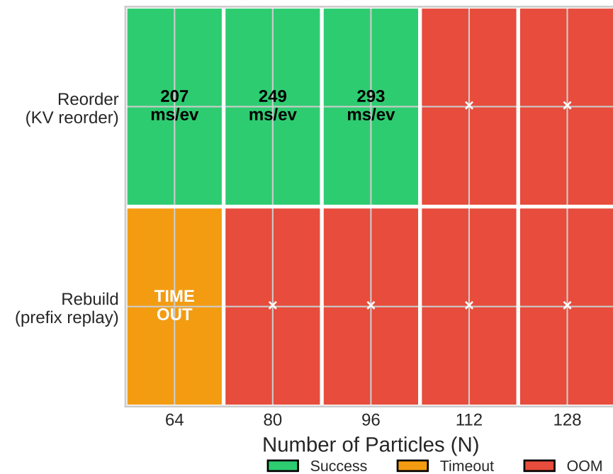
(c) Feasibility (L=3072, R=50)
