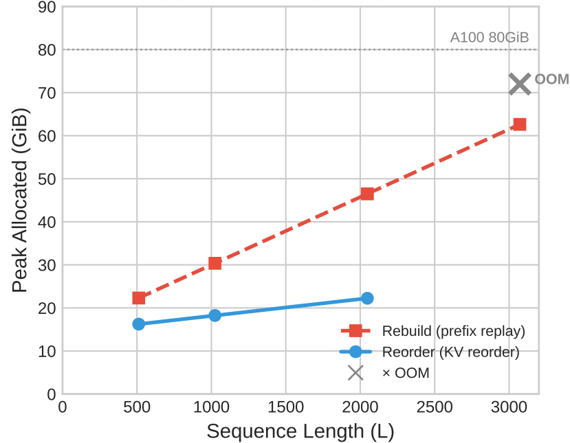
(b) Peak Memory vs L (N=64)
