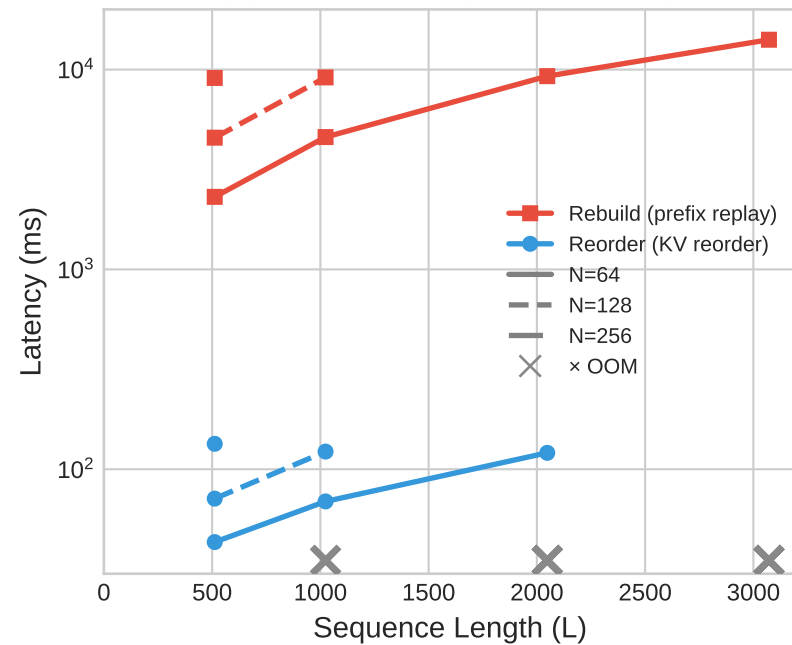
(a) Latency vs L (N=64/128/256)
