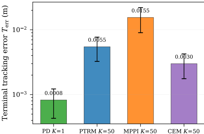
(a) Terminal tracking error
