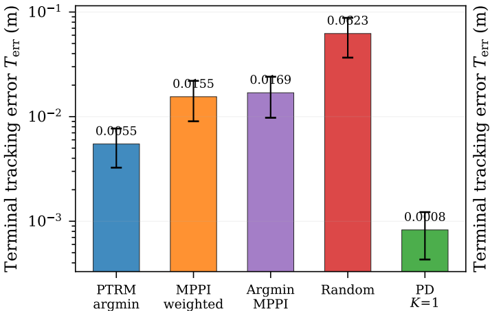
(a) Selection strategy
