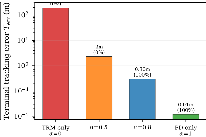
(b) Candidate generation ( \alpha ablation)
