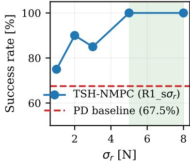
(a) Success rate
