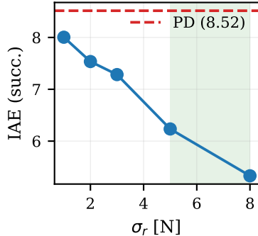
(c) Integral abs.\ error
