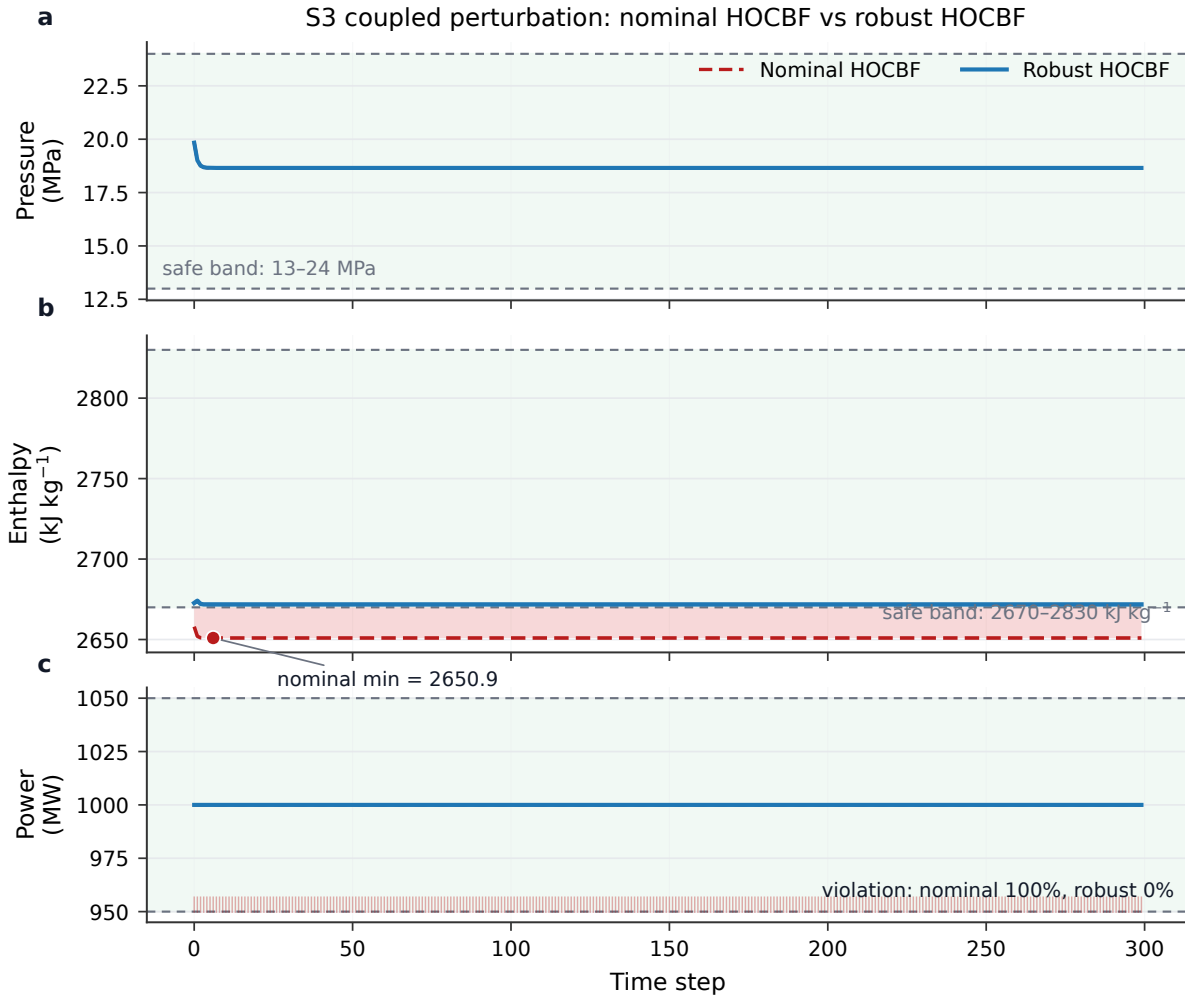
S3 coupled perturbation: nominal HOCBF vs robust HOCBF
