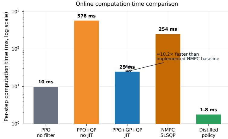
Figure S1: Per-step computation time comparison (log scale). PPO+GP+QP with JIT compilation (GPU): \sim 25 ms (p95: 27 ms); NMPC (CPU, SLSQP, N=10 horizon): 254 ms average.
