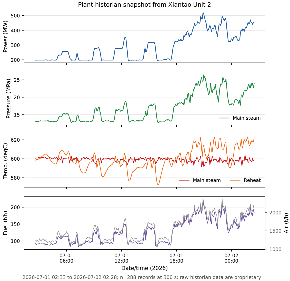
Figure 9: Plant-historian grounding from China Resources Xiantao Unit 2. The panels show five-minute samples of generator active power, main-steam pressure, main/reheat steam temperature, and fuel/air flow during a loaded operating interval. The record is used to ground measurement availability and operating variability; it is not a plant-trial evaluation of the proposed safety filter.
