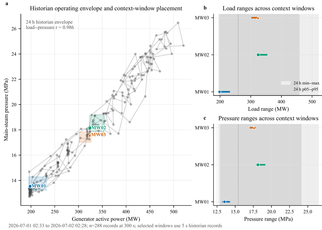
Figure 6. Plant-historian operating-envelope check from the 660 MW ultra-supercritical unit. (a) Five-minute historian samples define the measured load–pressure envelope over an approximately 24 h loaded interval; colored boxes and markers locate three two-hour post-retrofit low-to-mid-load historian windows. (b,c) The same windows are shown as load and pressure ranges against the 24 h min–max and p05–p95 envelopes. The figure places these historian windows within measured plant operation.
