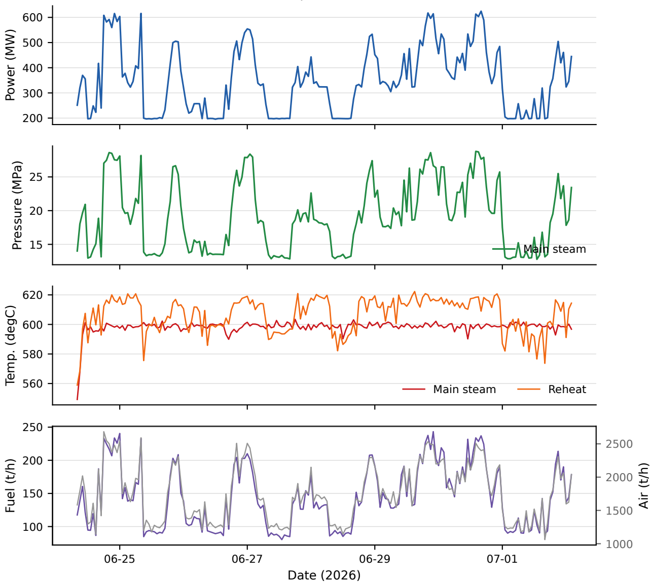
Plant historian snapshot from Xiantao Unit 2
