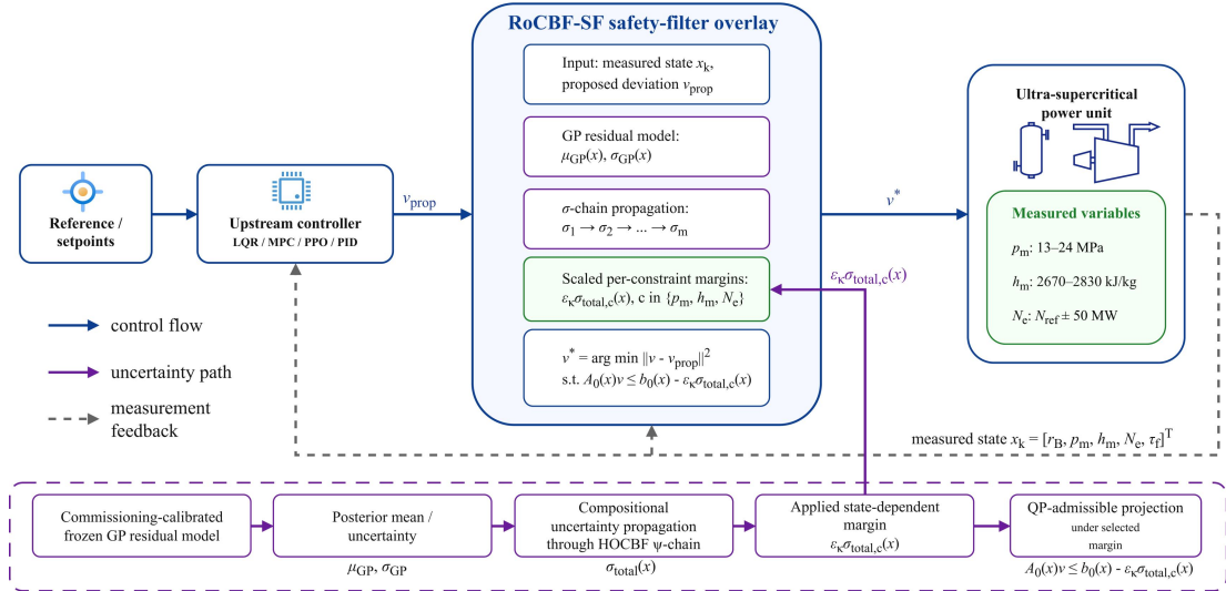
Figure 1. RoCBF-SF safety-filtering architecture. The upstream controller (LQR, MPC, PID, or learned policy) proposes a normalized deviation command v_{prop} . The filter evaluates that command against current plant measurements and the GP residual model, then projects it to the nearest QP-admissible deviation command v^* under A(x)v \leq b(x) - \epsilon_k \sigma_{total}(x) . The physical command is reconstructed with S_u by Eq. (1).
