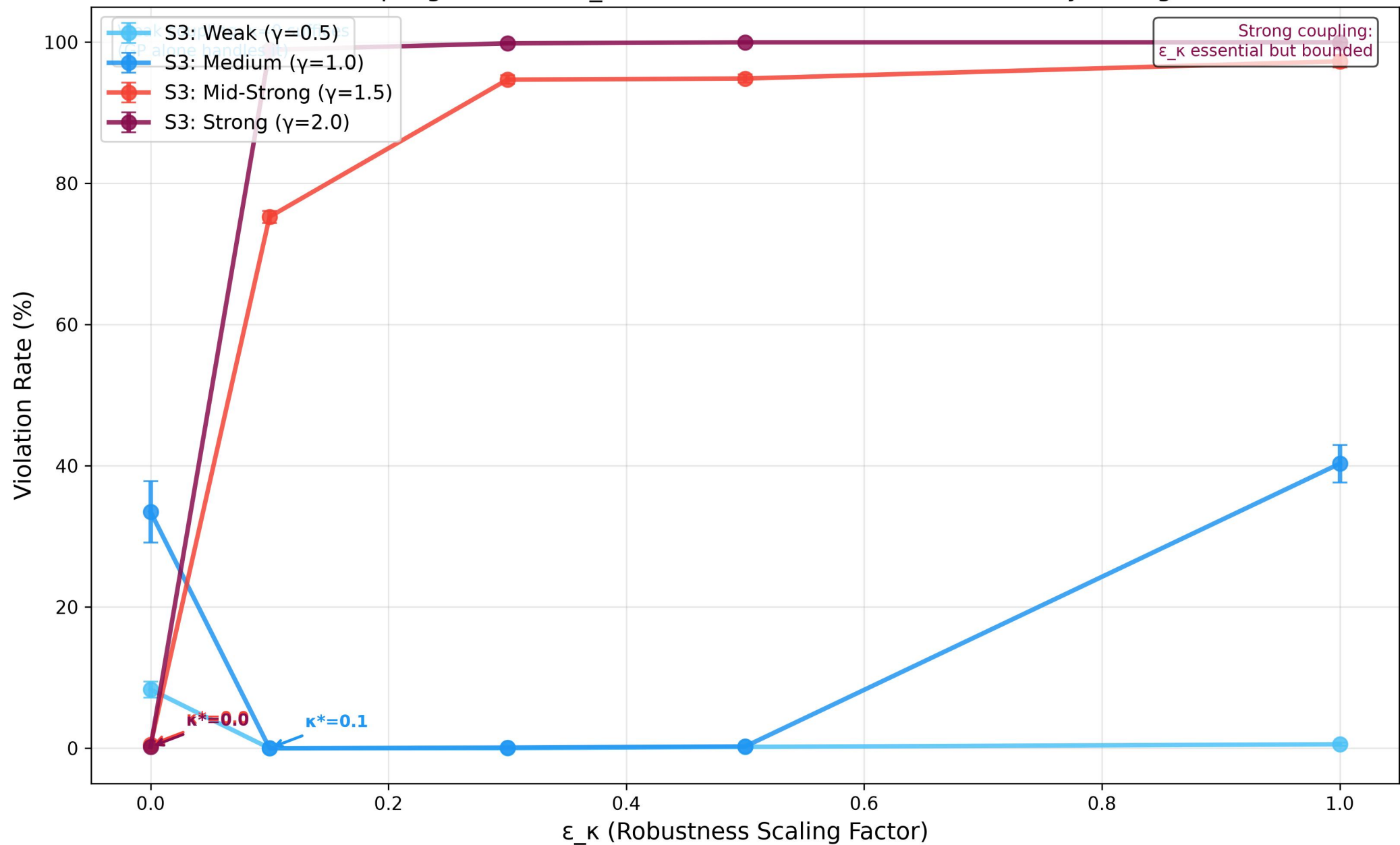
S3 Coupling Gradient: \varepsilon_\kappa Contribution Grows with Uncertainty Strength
