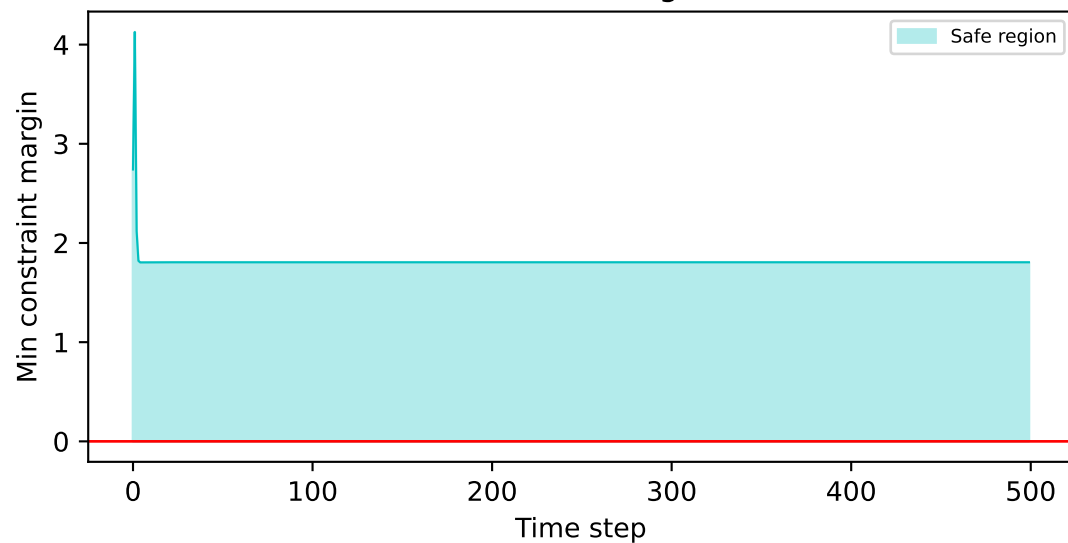
Minimum Constraint Margin (safe if >0)
