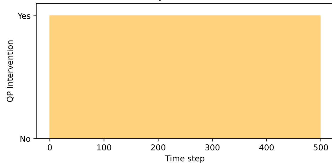
QP Safety Filter Intervention
