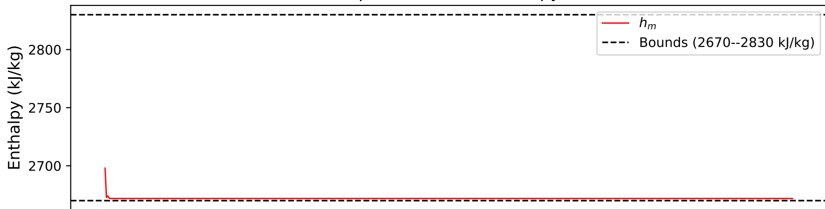
Separator Outlet Enthalpy
