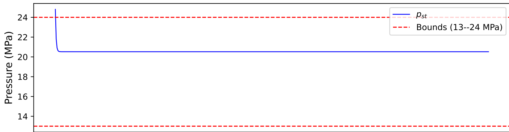
Main Steam Pressure
