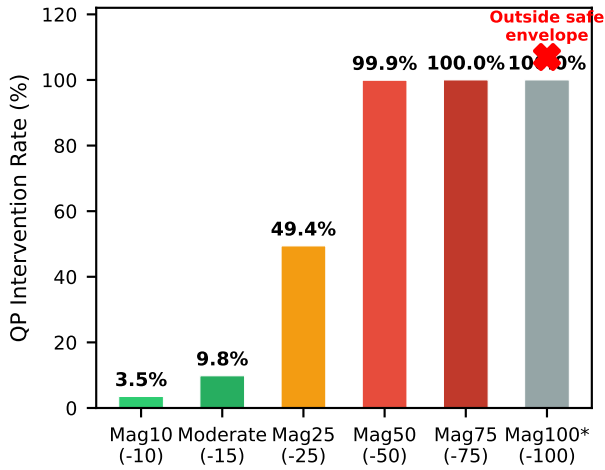
QP Filter Intervention vs. Perturbation Magnitude
