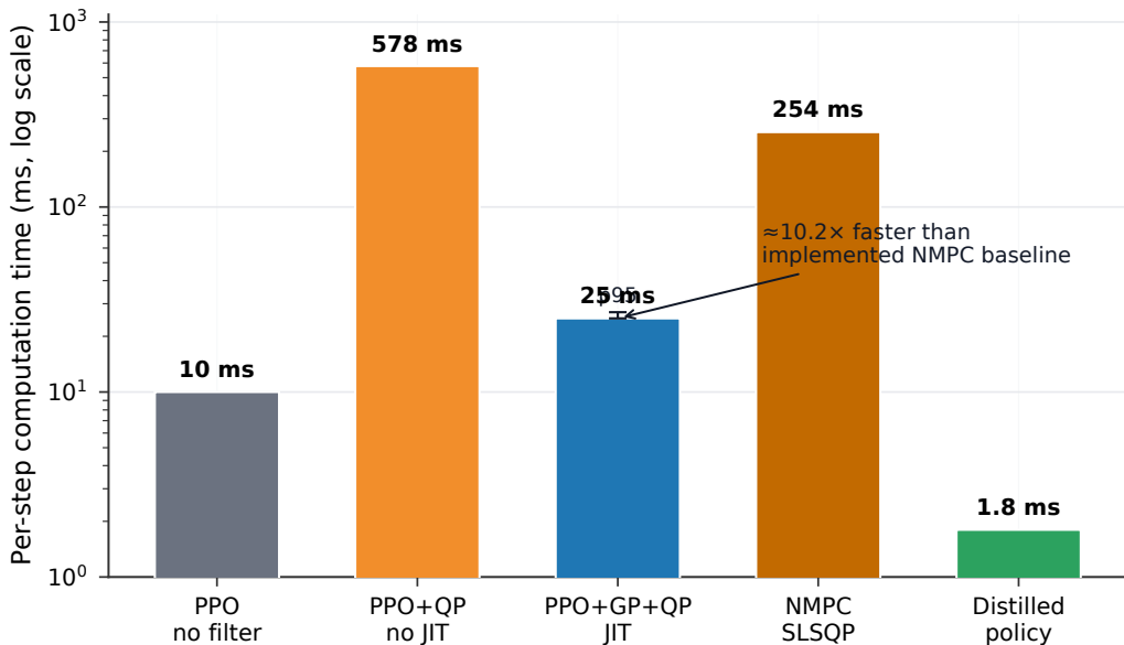
Online computation time comparison
