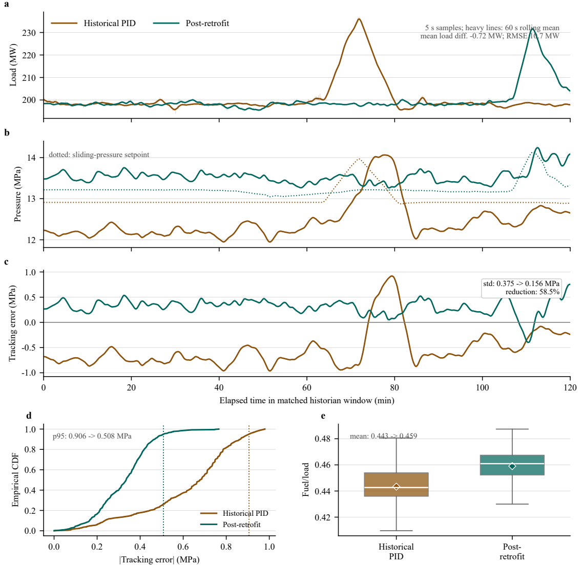
Figure 7: Matched plant-historian retrofit-window diagnostic from the 660 MW ultra-supercritical unit. The historical PID window is 5 November 2025 11:00–12:59:55 local time; the post-retrofit window is 25 June 2026 12:30–14:29:55 local time. Both windows contain 1440 original 5 s historian samples. (a) Generator active-power trajectories used for matching; the mean-load difference is -0.72 MW and the load-profile RMSE is 10.7 MW. (b) Main-steam pressure and the sliding-pressure setpoint. (c) Pressure tracking error, p_{\text{main}} - p_{\text{set}} ; the sample-level standard deviation decreases from 0.375 to 0.156 MPa. (d) Empirical CDF of absolute pressure tracking error; dotted lines mark the 95th percentile, which decreases from 0.906 to 0.508 MPa. (e) Fuel/load distribution for the combustion-side operating context; boxes show median, IQR, and 1.5 \times \text{IQR} whiskers, and diamonds show means. Light traces are original samples and heavy traces are 60 s rolling means for readability; all reported metrics use the original 5 s samples.
