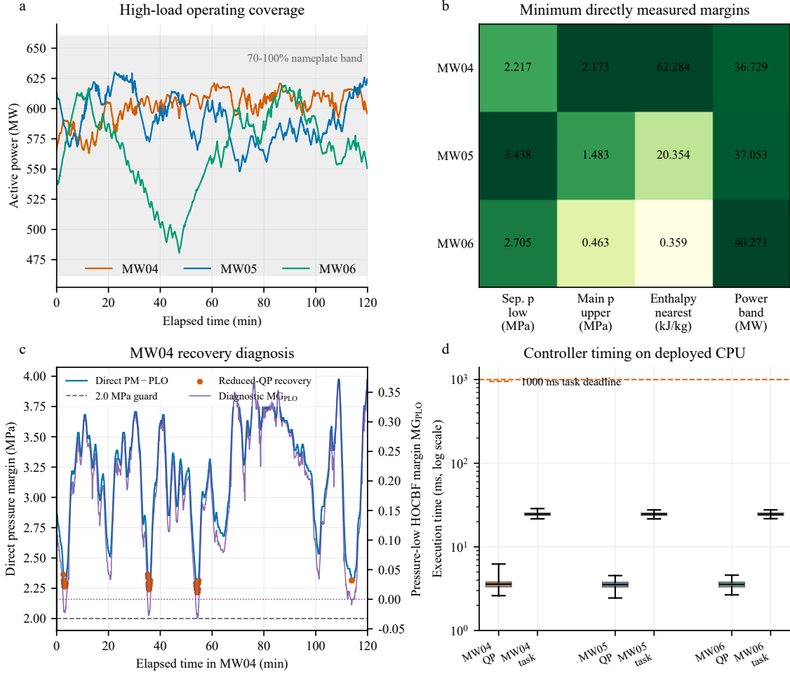
Figure 8: High-load plant-controller evidence from three post-retrofit two-hour windows, each containing 1440 records exported at 5s spacing from a controller executing at 1s. (a) Generator active power; the shaded band denotes 70–100% of the 660 MW nameplate rating. (b) Minimum directly measured margins to the separator-pressure lower bound, main-steam-pressure upper replay bound, nearest separator-enthalpy bound, and \pm 50 MW power band. Cell shading is normalized within each column; annotations retain physical units. (c) MW04 recovery diagnosis: the directly measured separator-pressure margin remains above the 2.0 MPa guard while the pressure-low HOCBF diagnostic row becomes negative; orange markers denote the 43 one-retry reduced-QP records. (d) QP and total task execution times on the deployed CPU; whiskers span the observed ranges and the dashed line marks the 1000 ms task deadline.
